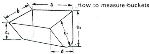
DIMENSIONS TABLE OF ELEVATORS BUCKETS
