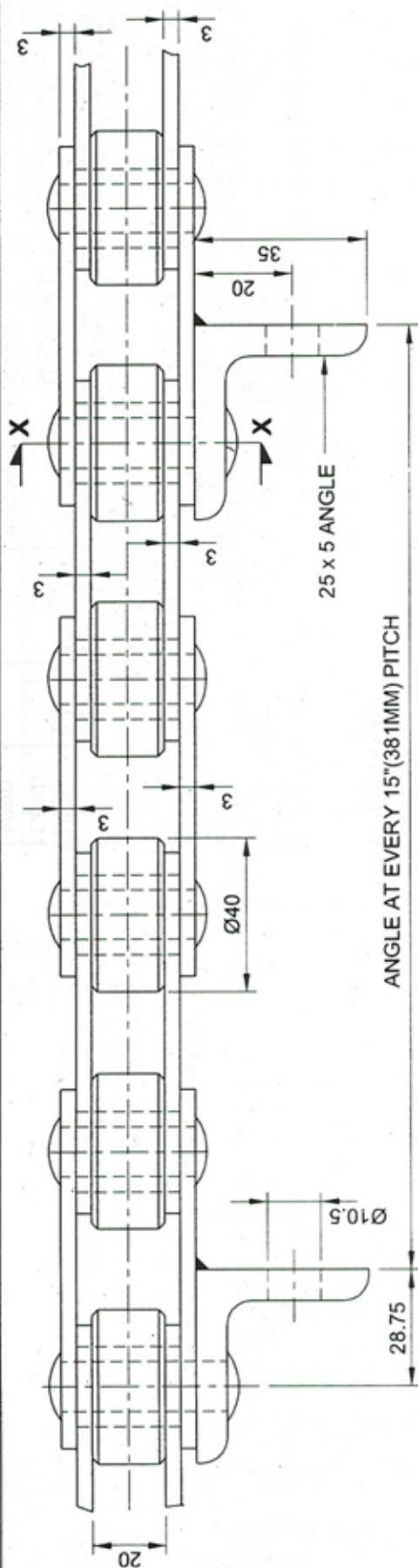
PLAN
