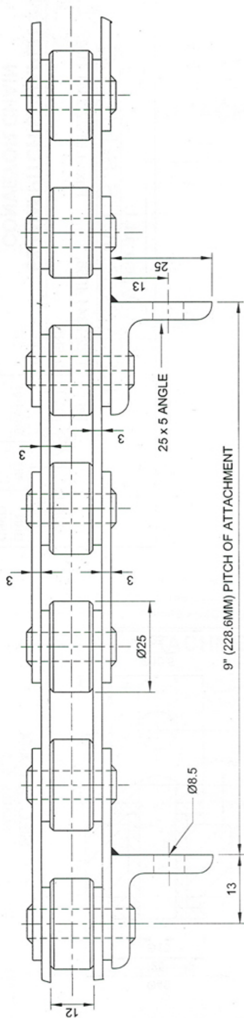
PLAN
